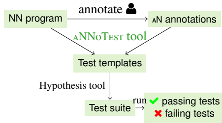
Figure 1: An overview of how the aNNoTEST approach works.
