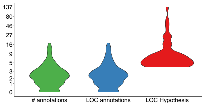
Figure 2: Distribution of the number of \Delta N annotations, lines of code (LOC) of \Delta N annotations, and LOC of generated Hypothesis templates for RQ1’s experiments.
